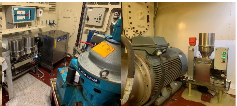
WP1-C1-1000 MGO/DO GreenOil fine filter system and WP2-H4-100 for the hvdralic fishing pump
